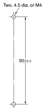
Mounting Holes
