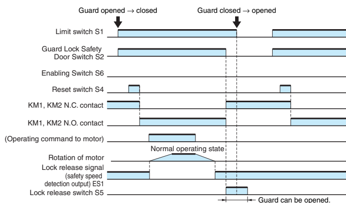
Timing Chart for Normal Operating Mode (M1: ON, M2: OFF)
